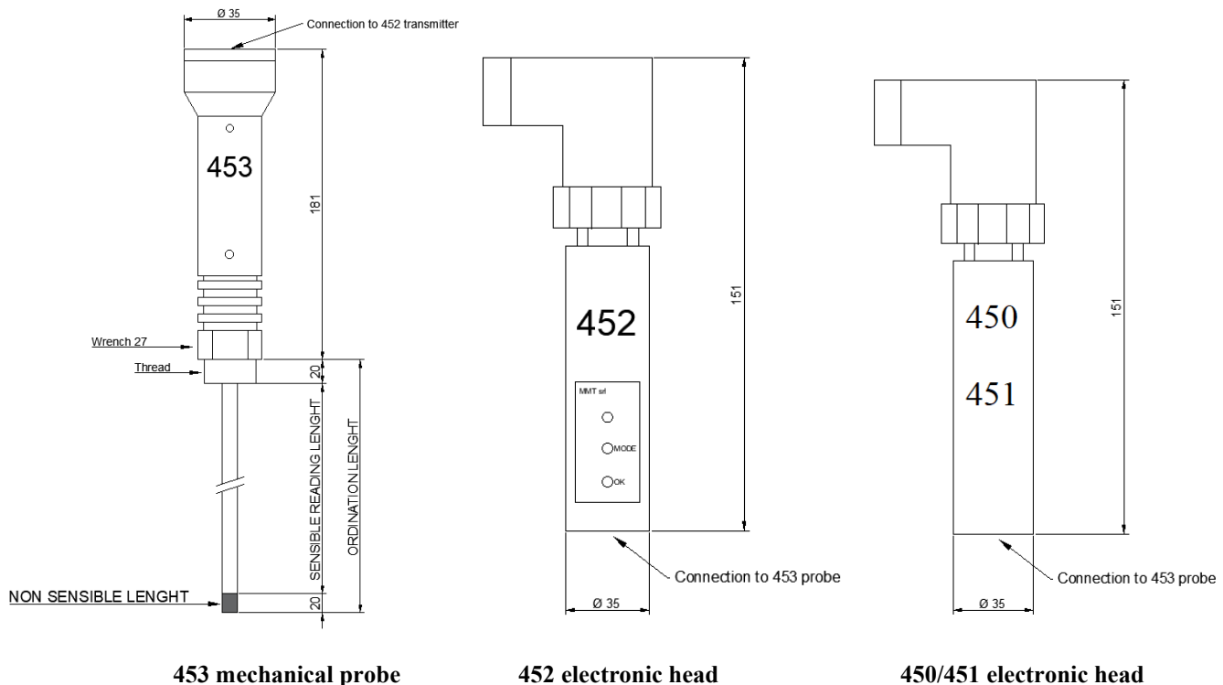
Drawing #1
