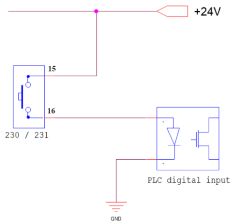
PNP
